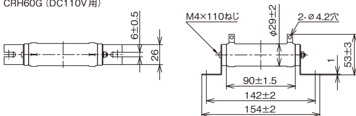
CRH60G (DC110V用)
