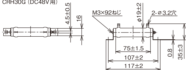
CRH30G (DC48V用)
